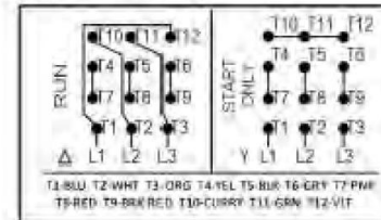
WYE-DELTA HIGH Voltage
