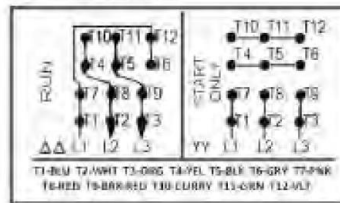
WYE-DELTA - LOW VOLTAGE
